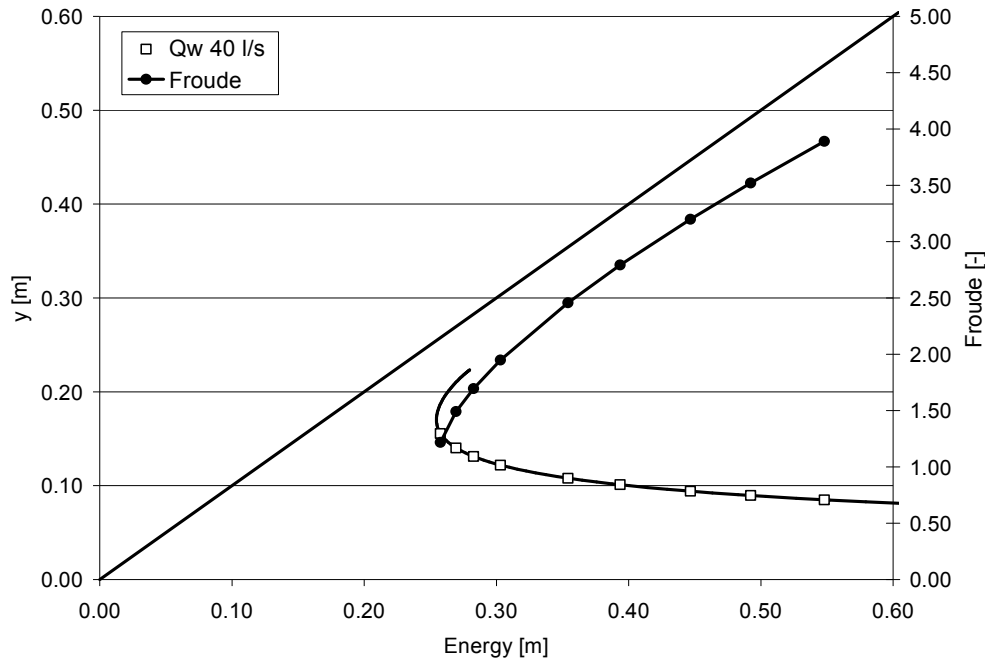
Figure 9. Specific energy curve and Froude for the 10 ° bend and 40 l/s
