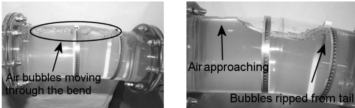
Figure 5. Left shows small air bubbles moving through the bend, Right shows an air pocket acting as buffer.
