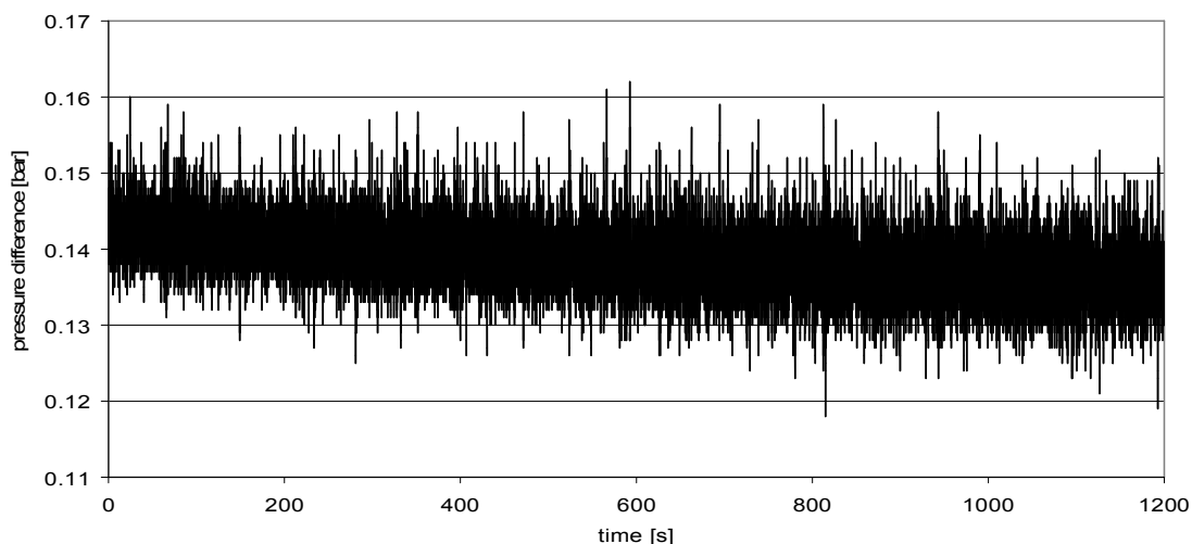
Figure 6. Air pocket growth over a period of 20 minutes
