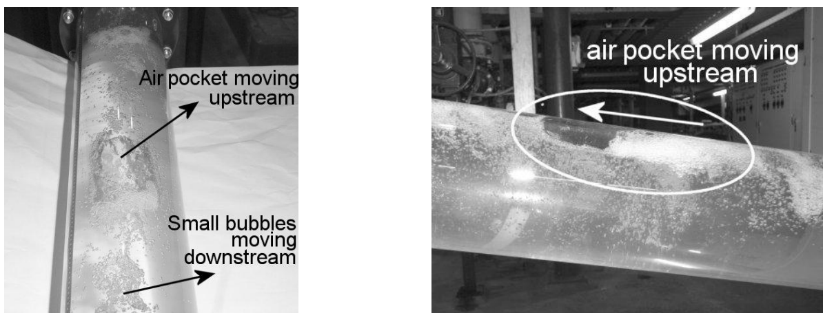
Figure 4. Dual mode flow, large plug moving upstream, small bubbles moving downstream.
